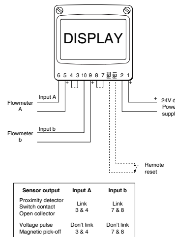
Fig 3 Typical measurement loop
