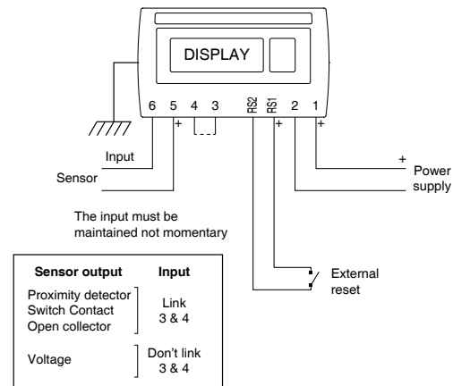
Fig 3 Typical system
