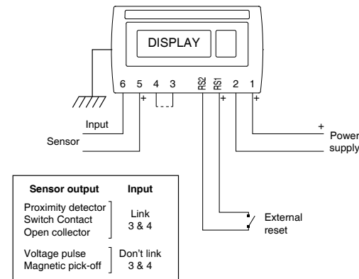
Fig 3 Typical system
