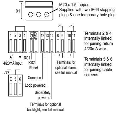
Fig 2 Dimensions and terminal connections
