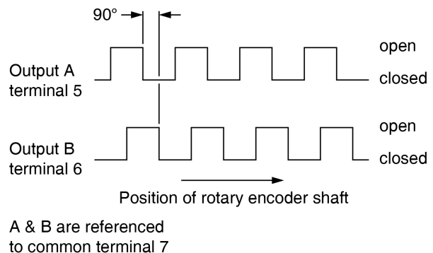
Fig 12 BA490 rotary encoder output waveforms
