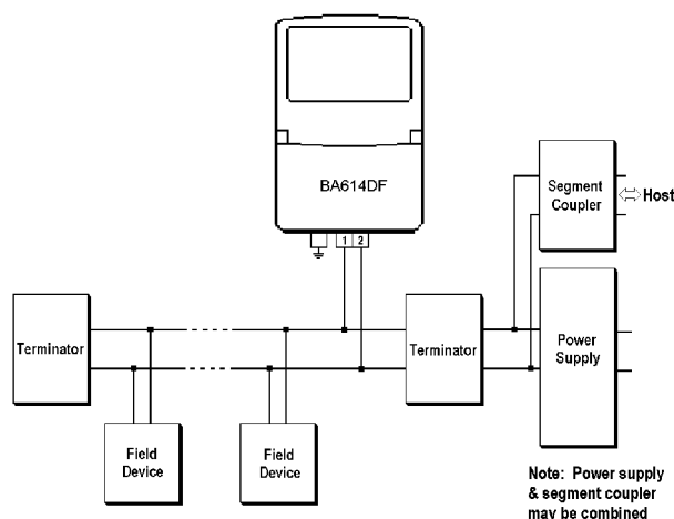
Fig 1 Fieldbus system
