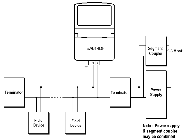
Fig 1 Fieldbus system
