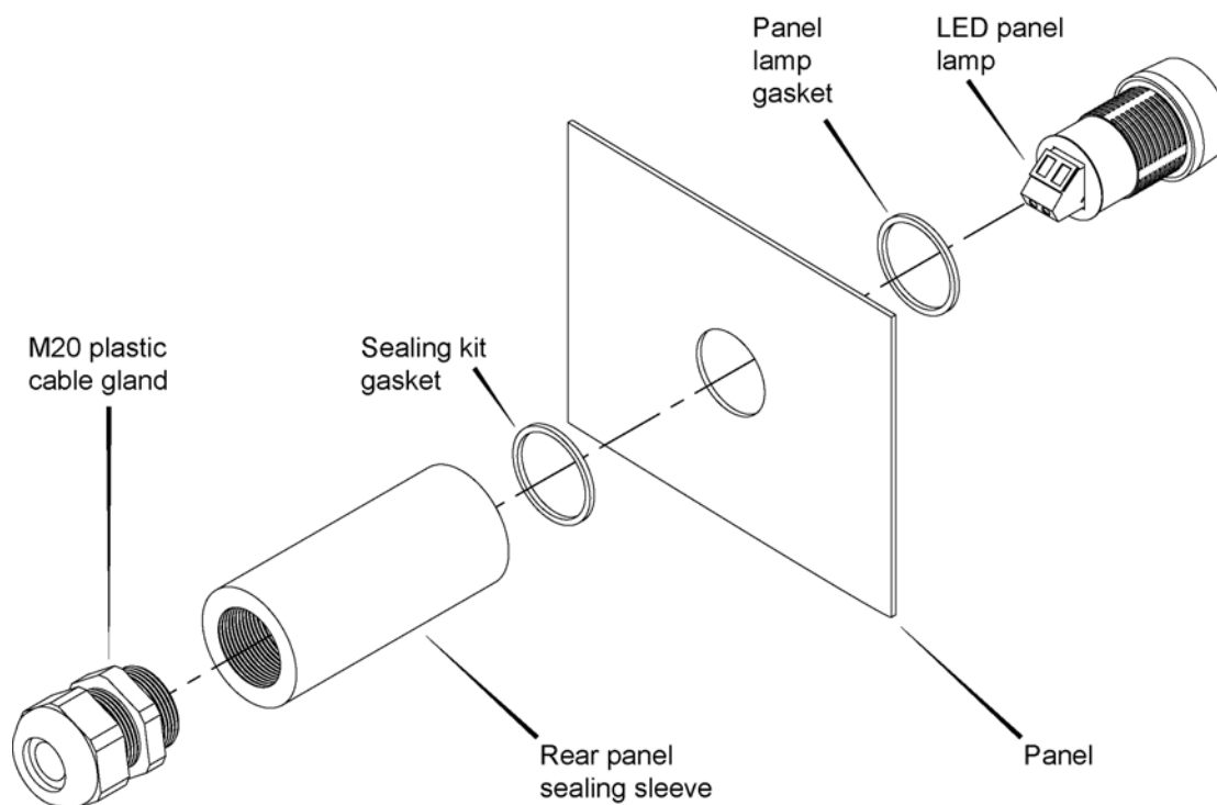
Fig 1 Assembly of BA599 rear panel sealing sleeve and LED panel lamp
