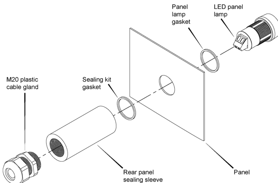
Fig 1 Assembly of BA590 rear panel sealing sleeve and LED panel lamp
