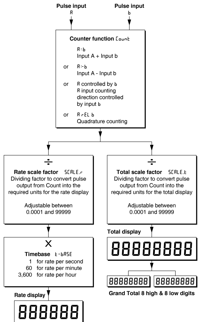
Fig 6 Calibration structure
