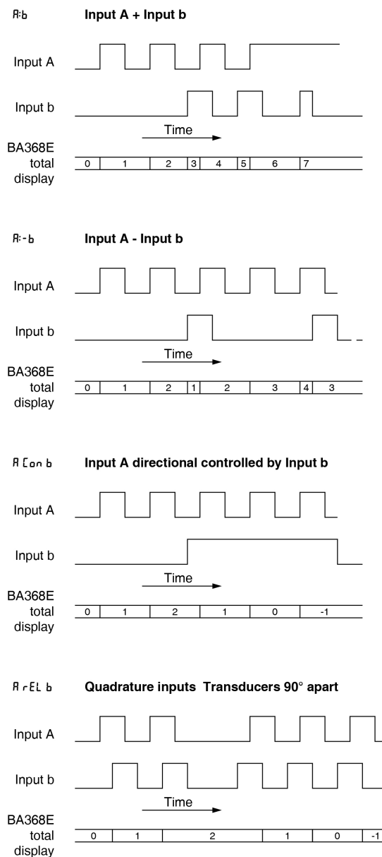
Fig 8 Counting waveforms
