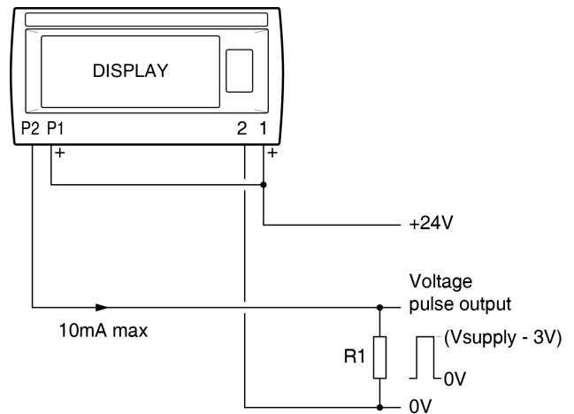
Fig 9 Generating voltage pulse in safe area using Zener barriers.
