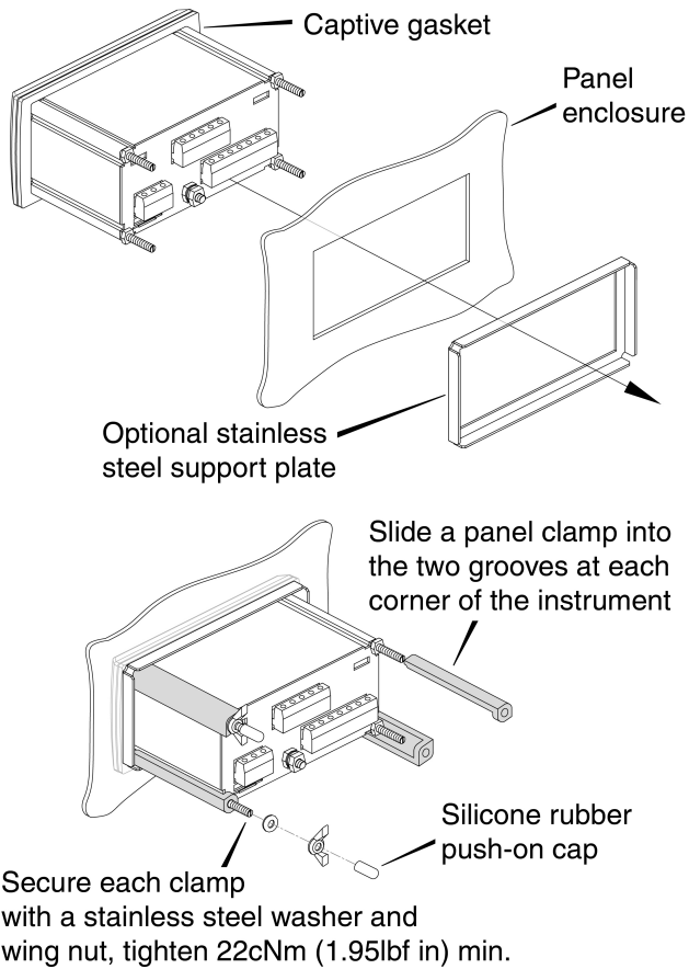
Fig 4 Installation procedure
