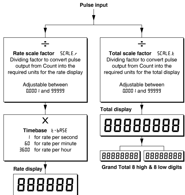
Fig 7 Calibration structure
