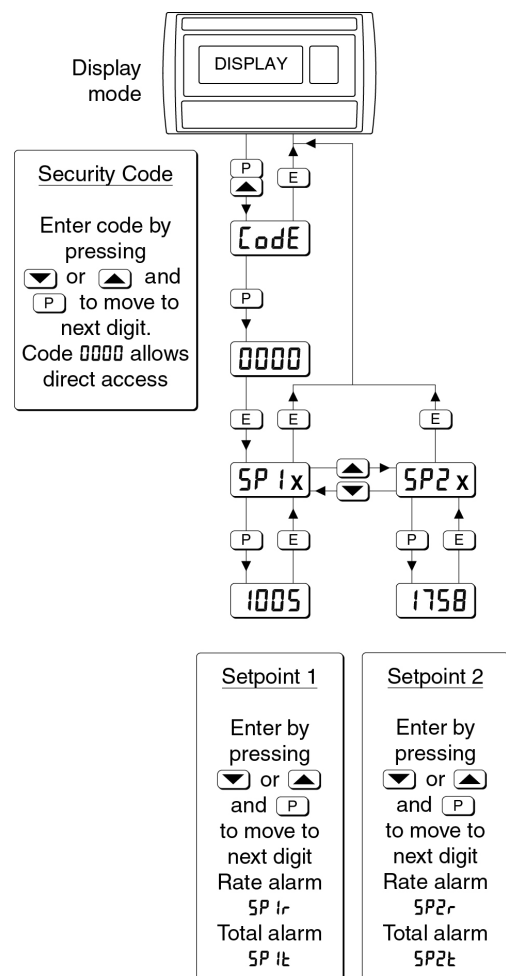
Fig 12 Setpoint adjustment from the display mode
