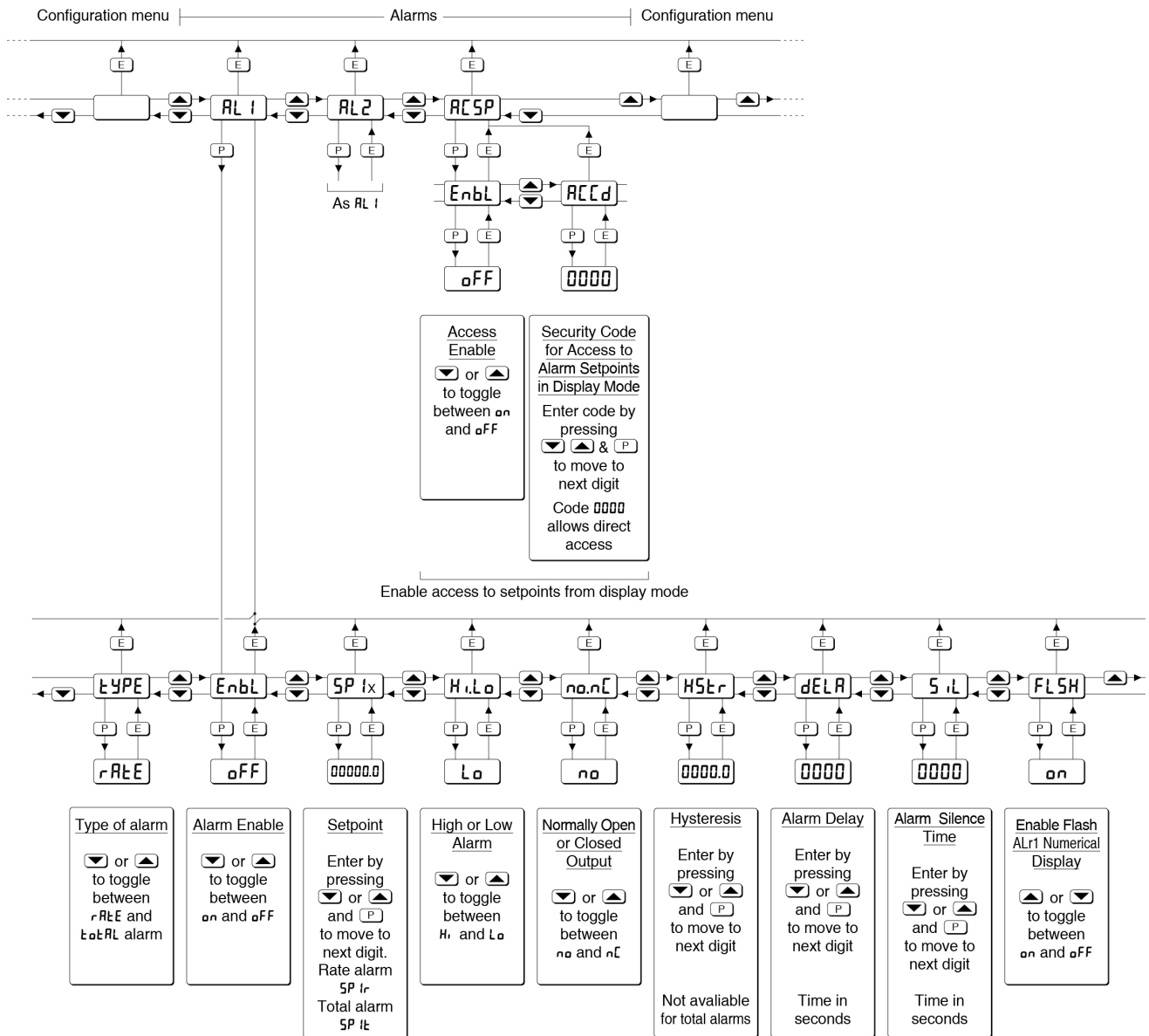
Fig 11 Alarm Configuration Functions in Configuration Menu
