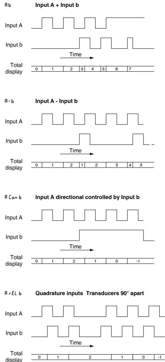
Fig 8 Counting waveforms
