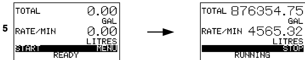
Shows batched quantity and units of measurement plus rate of dispensing and units of measurement.
