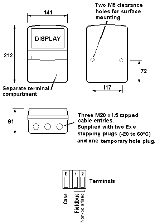
Fig 3 Dimensions and terminal connections
