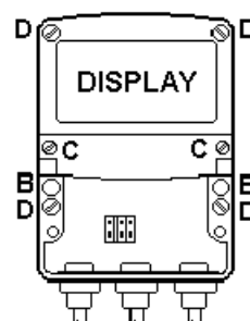
Fig 2 BA414NDF-F installation procedure
