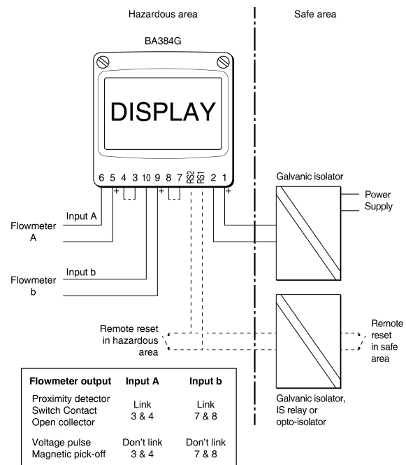
Fig 4 BA384G used with galvanic isolators
