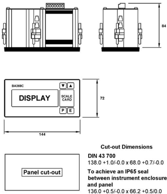
Fig 1.2 BA368C dimensions
