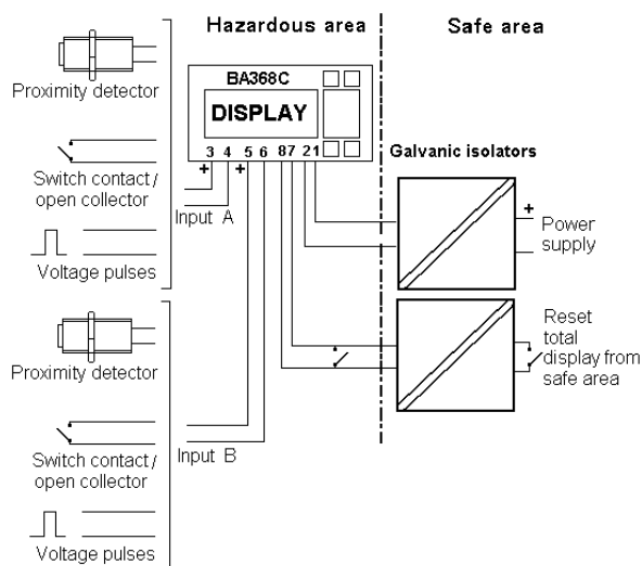
Fig 2.2 Basic counter circuit using isolators
