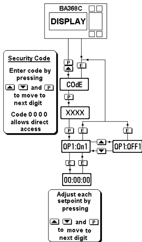
Fig 5.4 Setpoint adjustment from the clock display mode
