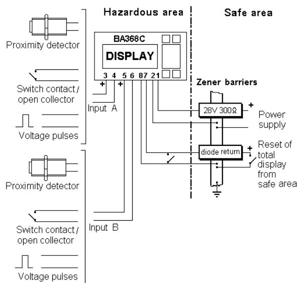
Fig 2.1 Counter installation using barriers
