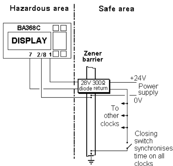
Fig 5.5 Clock application with synchronisation
