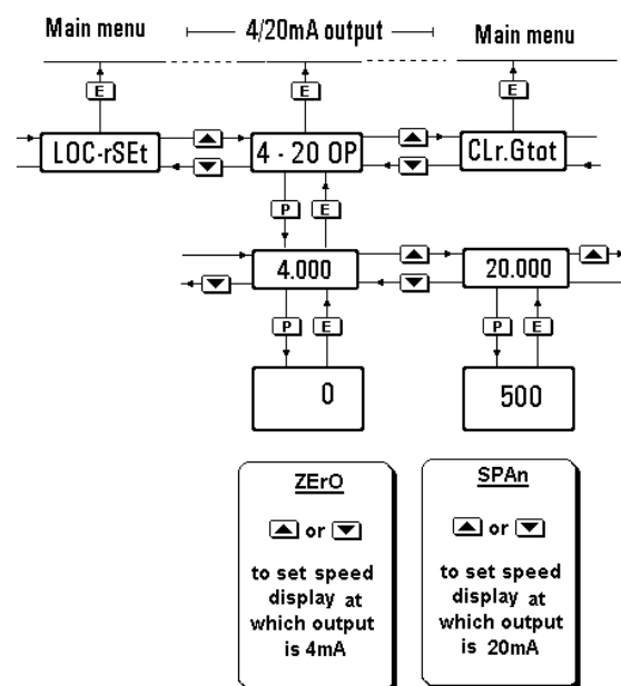
Fig 4.6 4/20mA output programme structure
