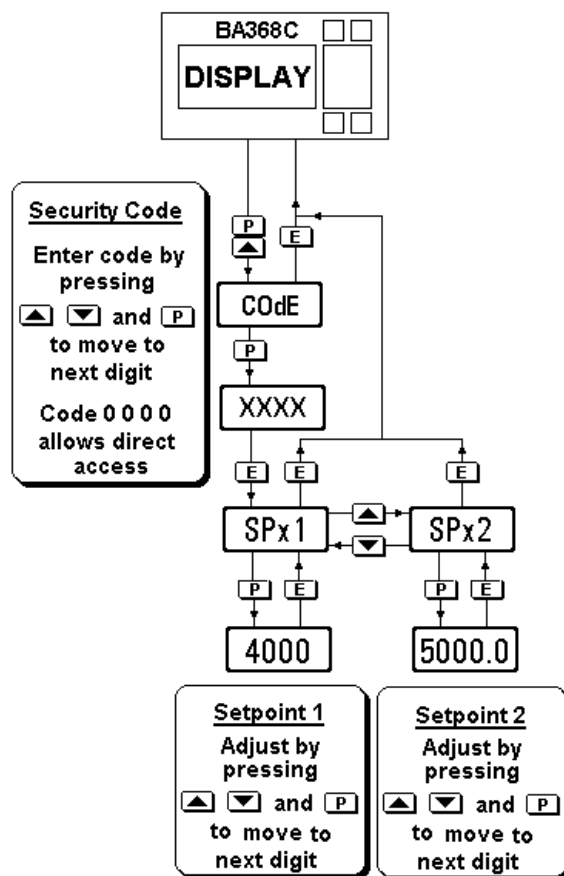
Fig 4.5 Setpoint adjustment from the display mode
