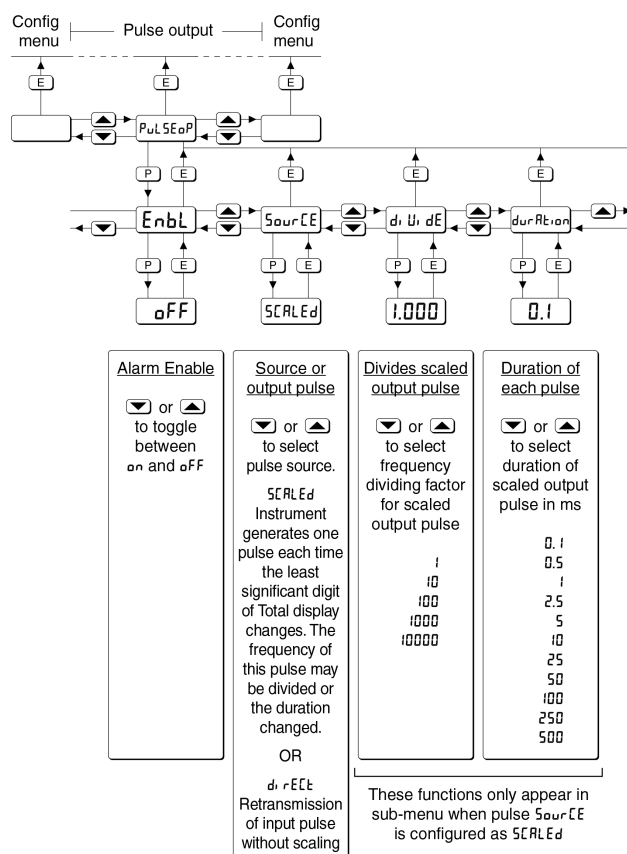
Fig 16 Pulse output configuration sub-menu
