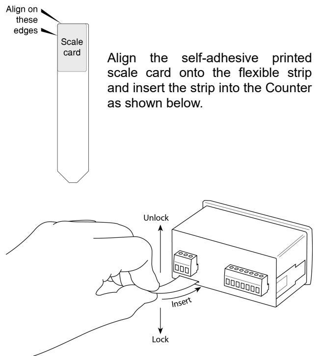
Fig 8 Inserting the flexible strip carrying the scale card into slot at the rear of the BA367E Counter.
