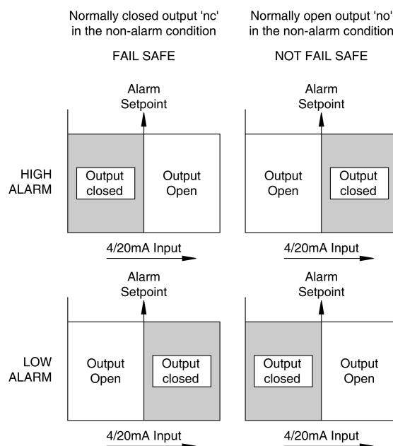
Fig 10 Alarm outputs
