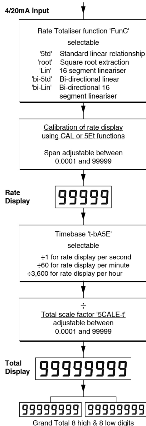
Fig 6 Calibration structure
