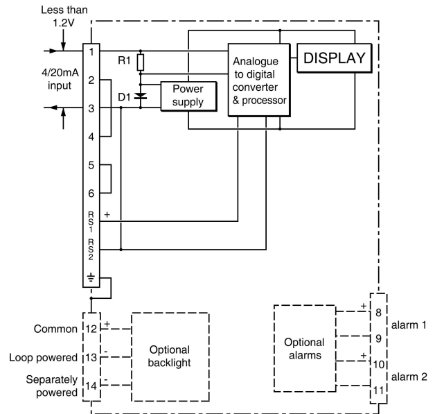
Fig 1 Simplified block diagram of BA354E
