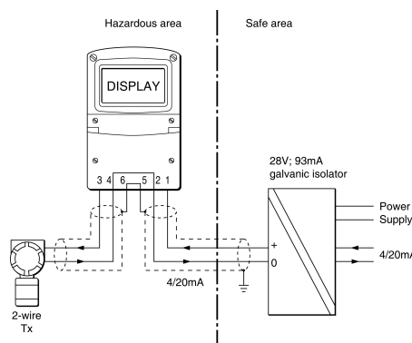
Fig 2b Loop powered by a galvanic isolator
