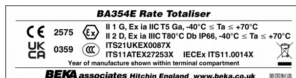
BA354E dust and gas certification label
