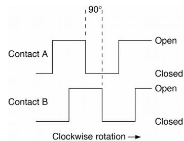
Fig 6 Quadrature sensor waveforms
