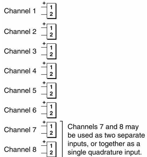
Fig 3 Input terminals
