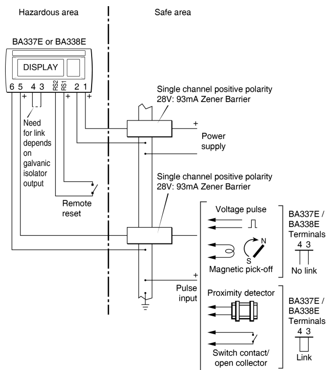
Fig 3 BA337E or BA338E used with Zener barriers pulse source in safe area.
