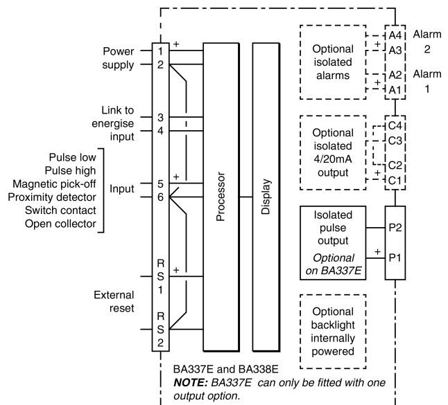
Fig 1 BA337E and BA338E block diagram
