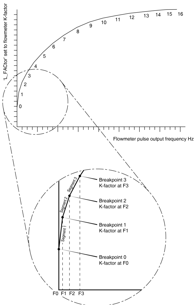
Fig 11 shows a typical linearising characteristic
