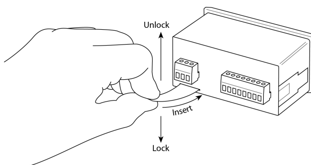
Fig 8 Inserting the flexible strip carrying the scale card into slot at the rear of Rate Totaliser.
