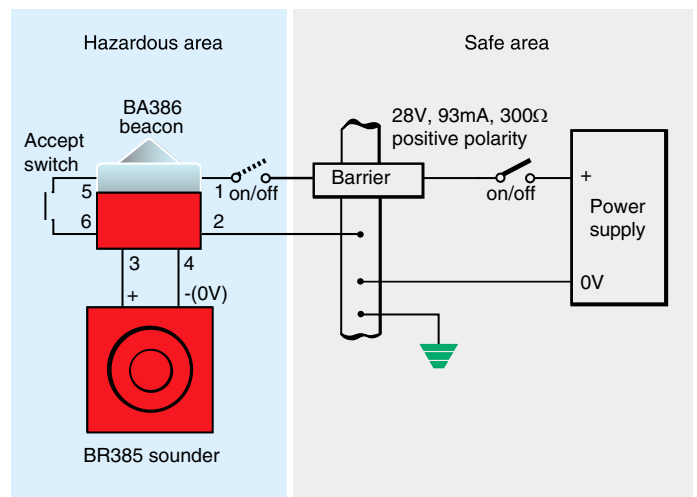
Fig 7 Combined circuit for BR385 sounder and BA386 beacon
