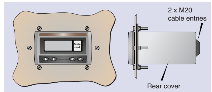
Fig 4 BA495 rear cover
