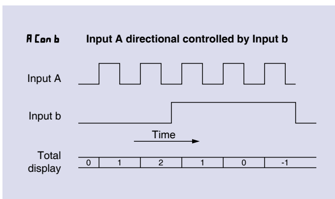
Fig 11b Input counting waveforms for input A controlled by input b.
